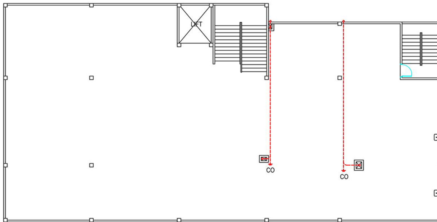
FOURTH FLOOR CEILING PLAN
