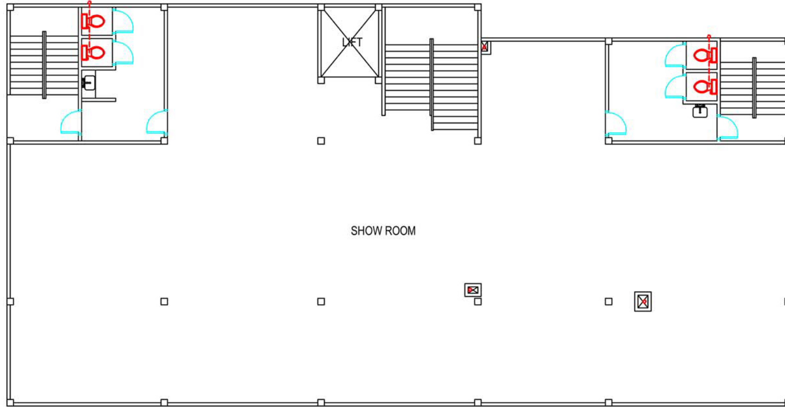
THIRD & FOURTH FLOOR PLAN
