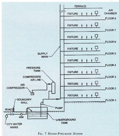
FIG. 7 HYDRO – PNEUMATIC SYSTEM
