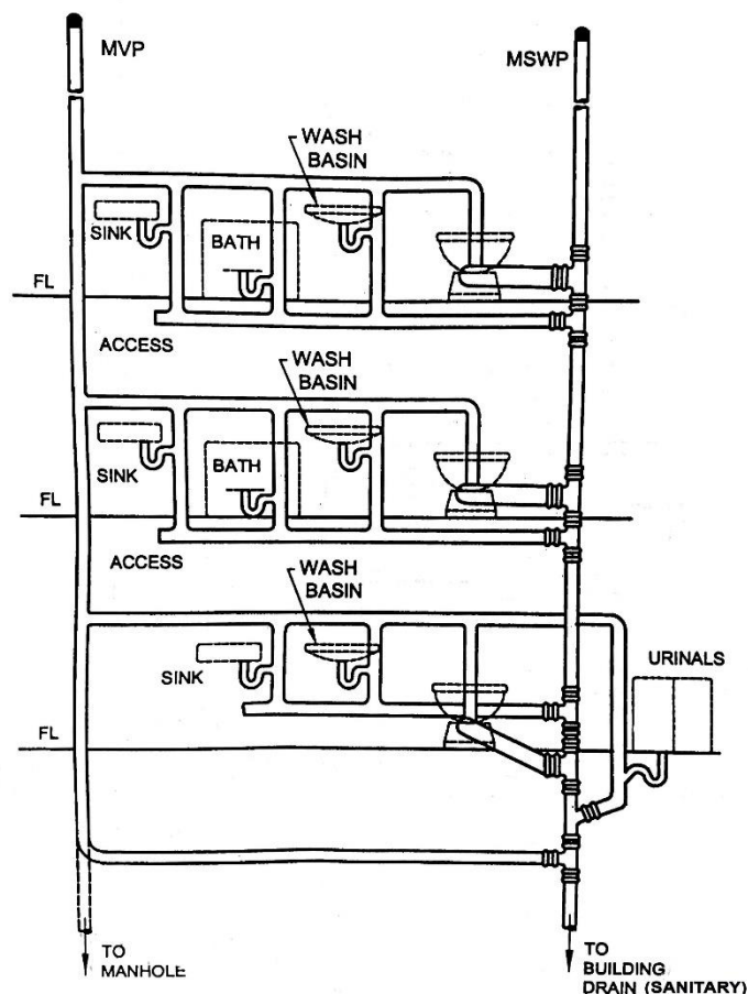
FIG.4 DIAGRAM OF ONE-PIPE SYSTEM
