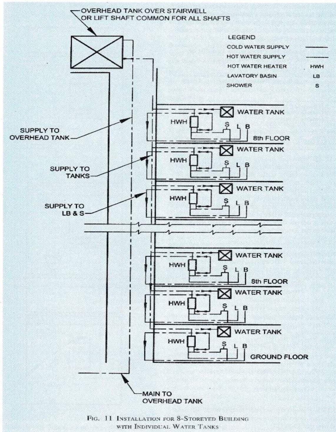
FIG. 11 INSTALLATION FOR 8 – STOREYED BUILDING WITH INDIVIDUAL WATER TANKS
