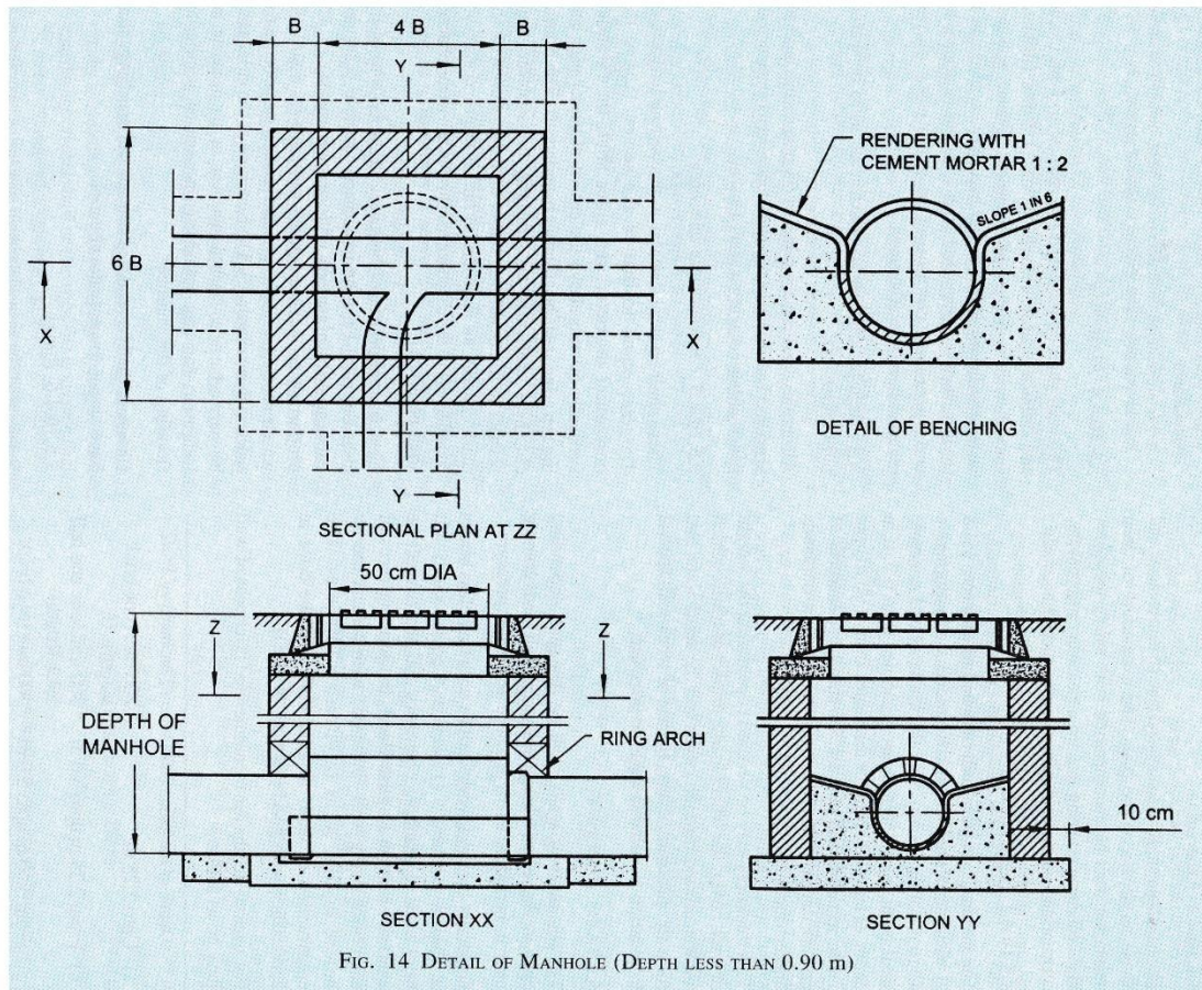
FIG. 14 DETAIL OF MANHOLE (DEPTH LESS THAN 3 FEET)
