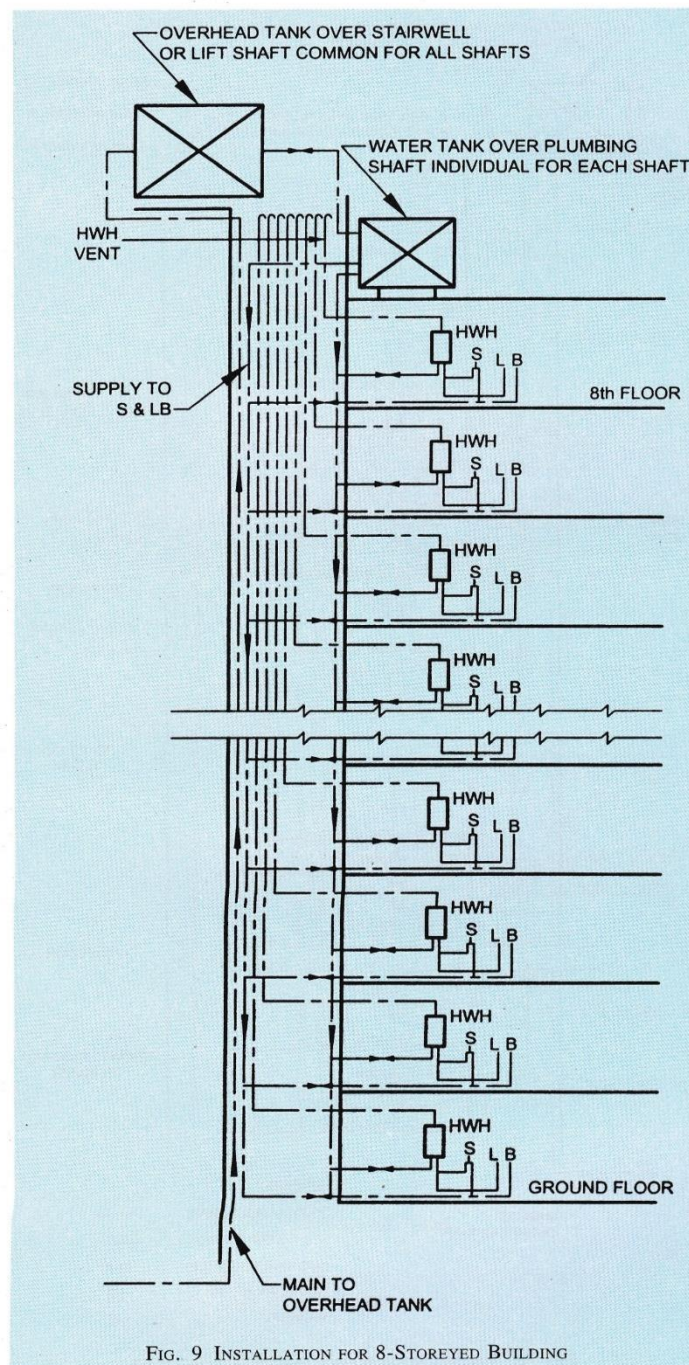
FIG. 9 INSTALLATION FOR 8 – STOREYED BUILDING
