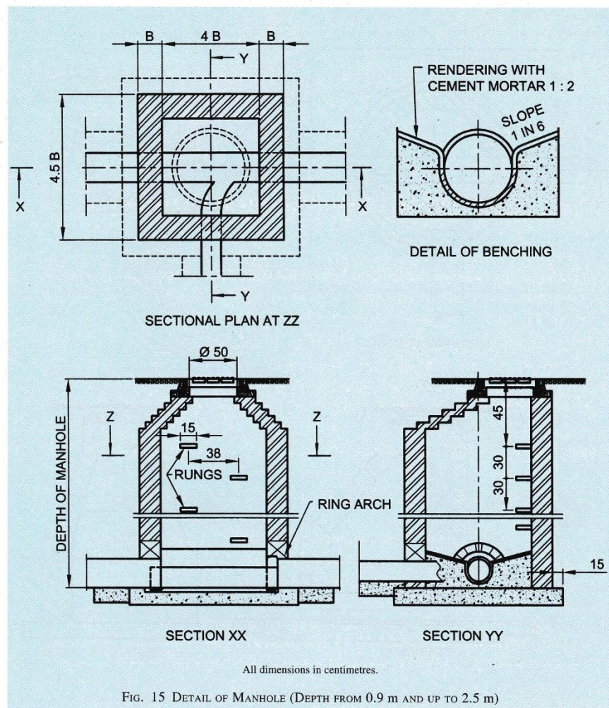
FIG. 15 DETAIL OF MANHOLE (DEPTH 3 FEET AND UP TO 8 FEET)
