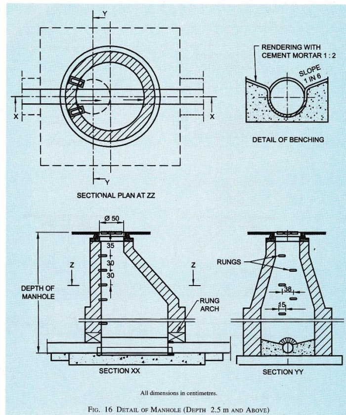
FIG. 16 DETAIL OF MANHOLE (DEPTH 8 FT AND ABOVE)
