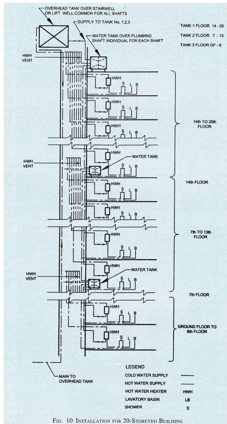
FIG. 10 INSTALLATION FOR 20 – STOREYED BUILDING
