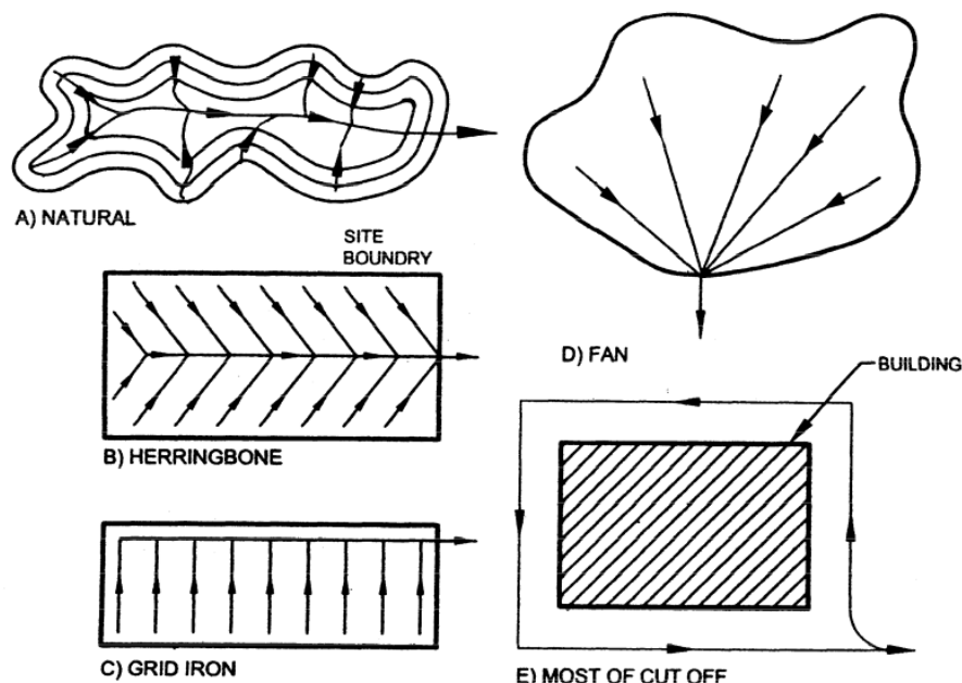
FIG. 19 DETAILS OF DRAINAGE SYSTEM
