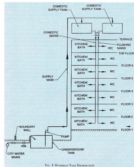
FIG. 8 OVERHEAD TANK DISTRIBUTION
